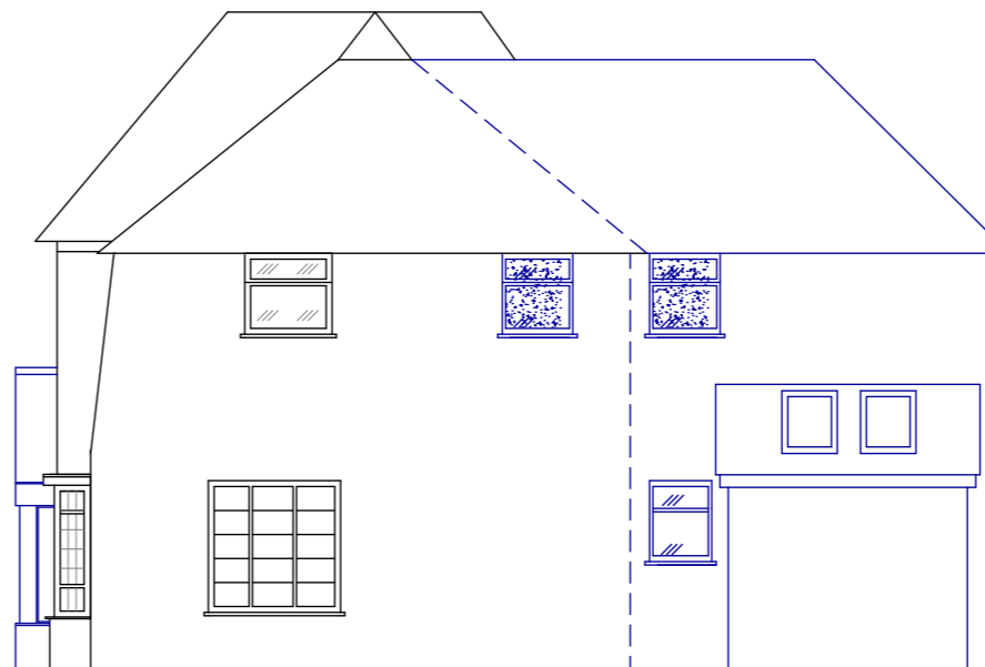
Right Elevation - Proposed
